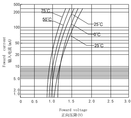
Forward current VS. Forward voltage 输入电流-正向压降曲线
