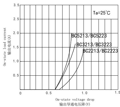
On-state load current VS. On-state voltage drop 输出电流-导通电压降曲线
